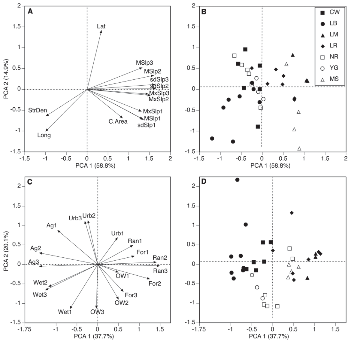
Figure 2. Principal component analysis (PCA) of continuous variables used in our study. A.—Multivariate relationships among physiographic variables. B.—Ordination of sampling sites in the physiographic PCA. C.—Multivariate relationships among land use/land cover (LULC) variables. D.—Ordination of the sampling sites in the LULC PCA. See Table 1 for abbreviations.
